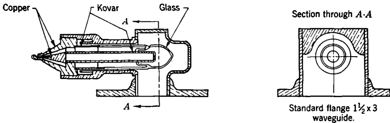
Fig. 11-17.—8.5-cm, 800-kw pulse-power "probe" transition for coaxial line to 1\frac{1}{4} - by 3-in. waveguide.
